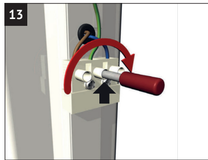
Tighten the 3 screws securing the cables. (Tighten the screws to 0,5 Nm.)
