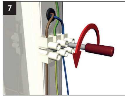
Loosen the 3 screws to remove the cables.
